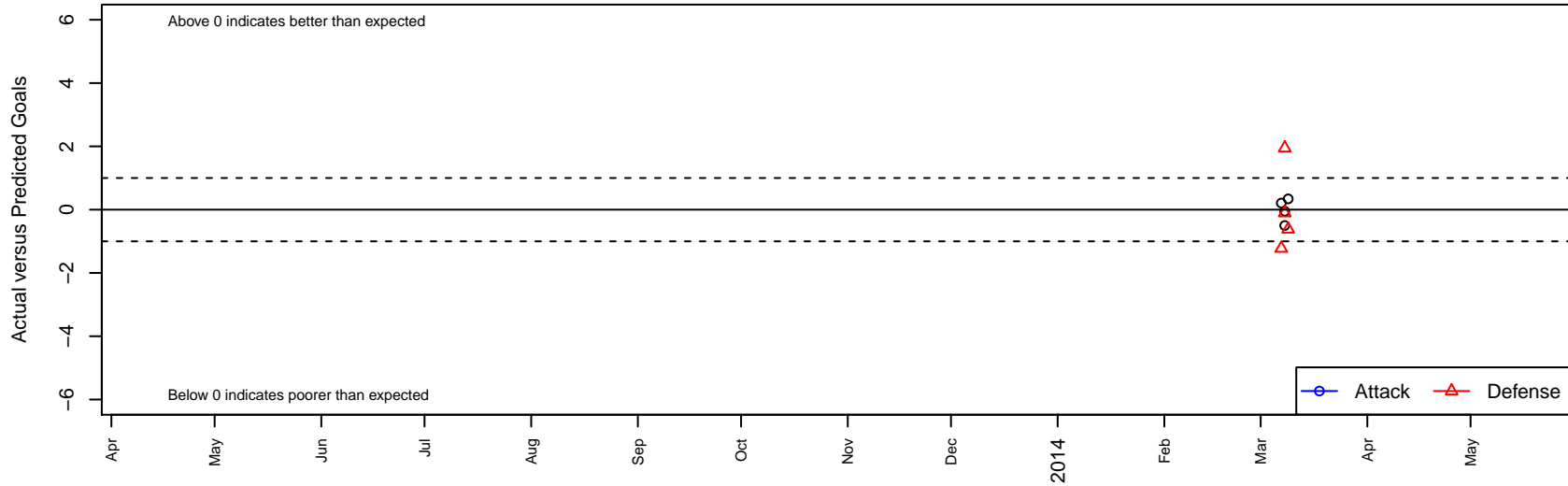
Legacy Football 99 B98 Dots are actual minus expected GF (blue circles) and GA (red triangles). Blue line is smoothed change in attack strength. Red is smoothed change in defense strength.
